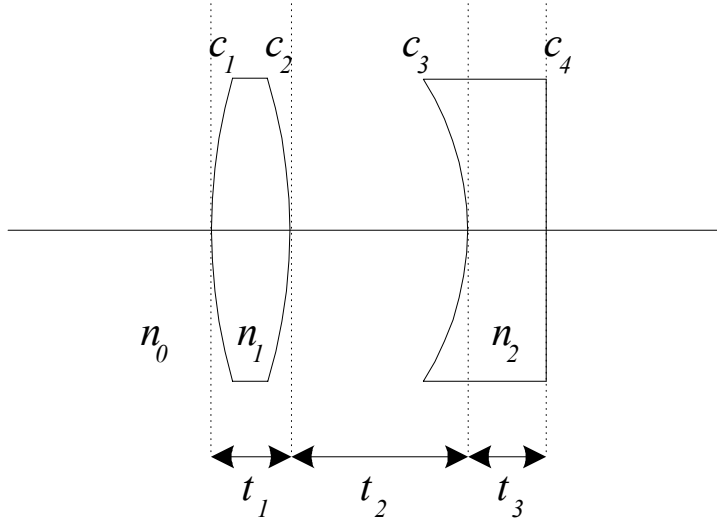
Figure 1: Parameters of a two-lens system: n_j represents the refractive index of a media, c_j a lens surface curvature, t_1 and t_3 are the lens thicknesses, and t_2 is the lens spacing.
