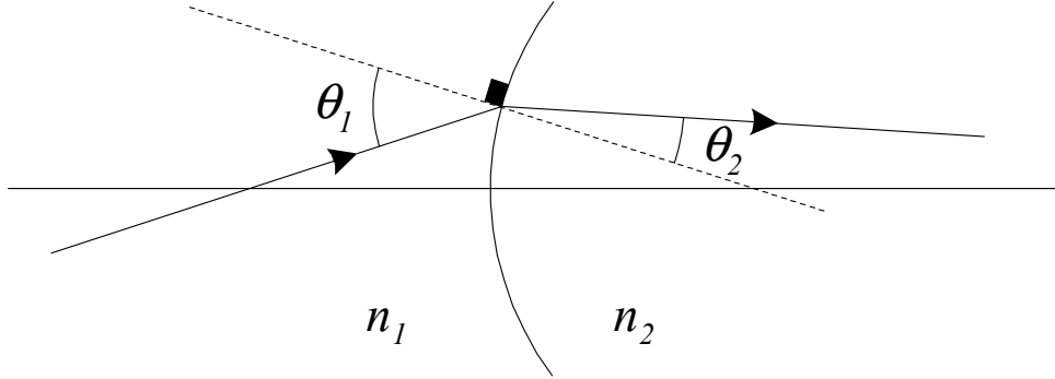
Figure 2: Illustration of Snell-Descartes first law of refraction.
